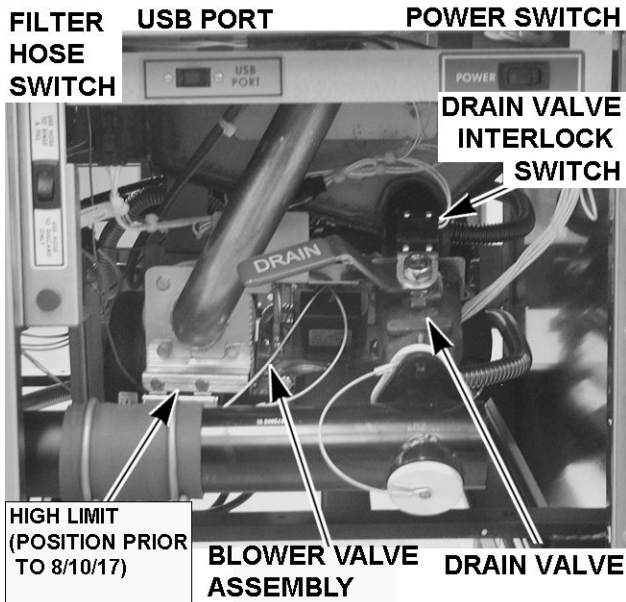
POWER SUPPLY BOX - RIGHT SIDE OF EACH FRYER SECTION 24872
